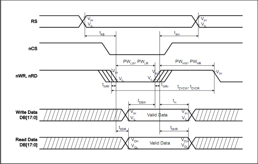
Reset Timing Characteristics (IOVCC = 1.65 ~ 3.3 V)
