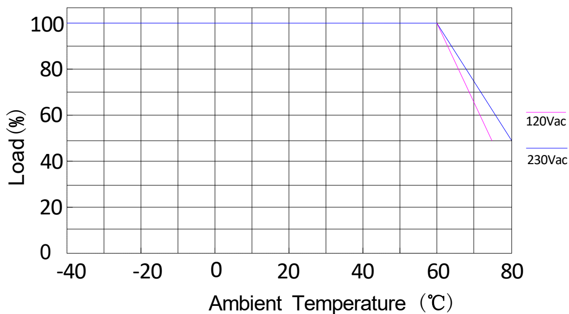
Derating Curve
