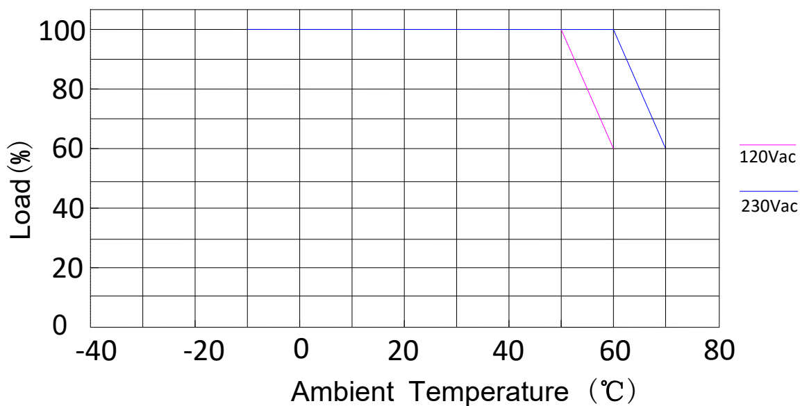
Derating Curve
