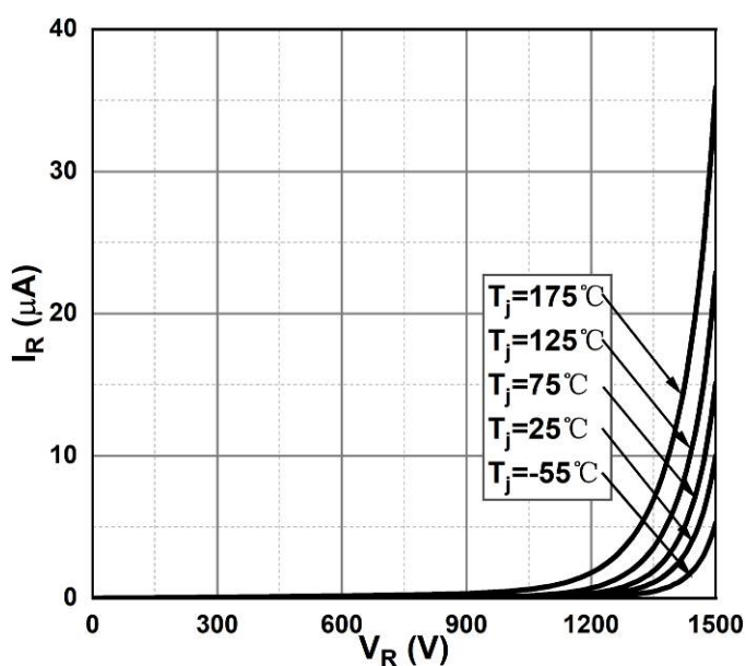
Figure 2. Reverse Characteristics
