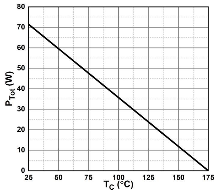
Figure 6. Power Derating
